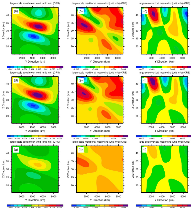
Fig. 1: The two horizontal wind components (left and middle column) and the vertical wind (right), all in m/s, induced by a GW packet, as simulated by PincFloit LES (top row), the WKB MS-GWaM according to Achatz et al (2017, middle), and the conventional WKB approach (bottom), taken from [9].
