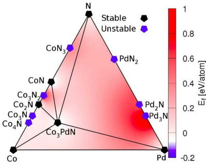
Figure 1: Ternary phase diagram of Co-Pd-N.
