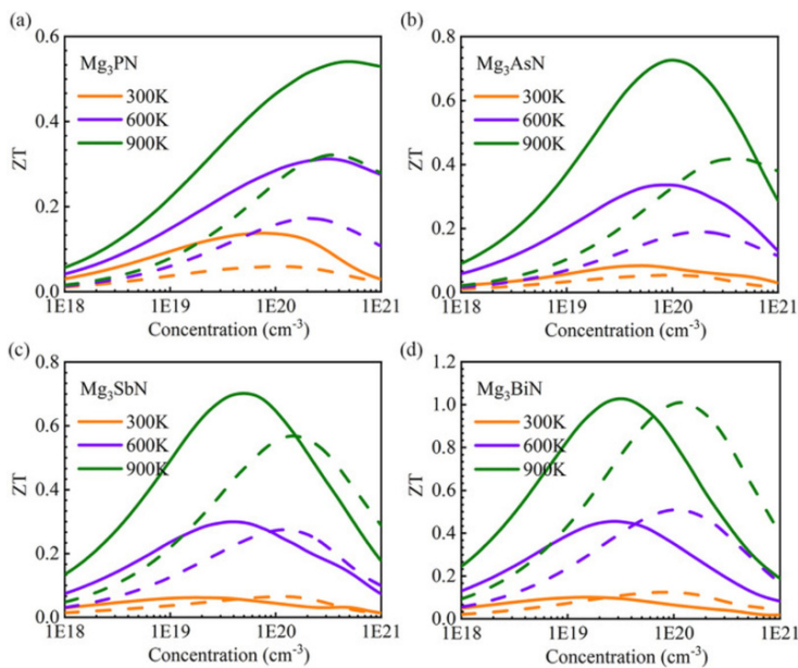
Figure 1: The thermoelectric figure of merit ZT as a function of carrier doping concentration of (a) Mg 3 PN, (b) Mg 3 AsN, (c) Mg 3 SbN, and (d) Mg 3 BiN at 300, 600, and 900 K
